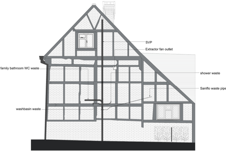
NORTH ELEVATION AS PROPOSED 1:50 scale
