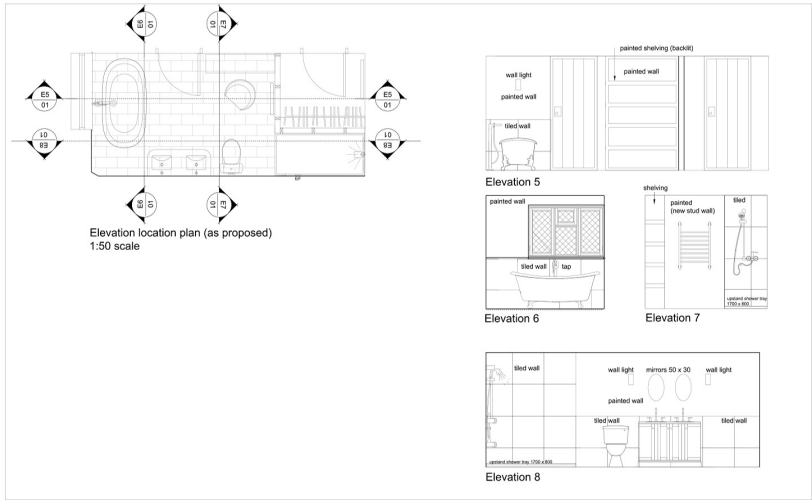
INTERNAL ELEVATIONS (FIRST FLOOR BATHROOM) AS PROPOSED 1:50 scale
