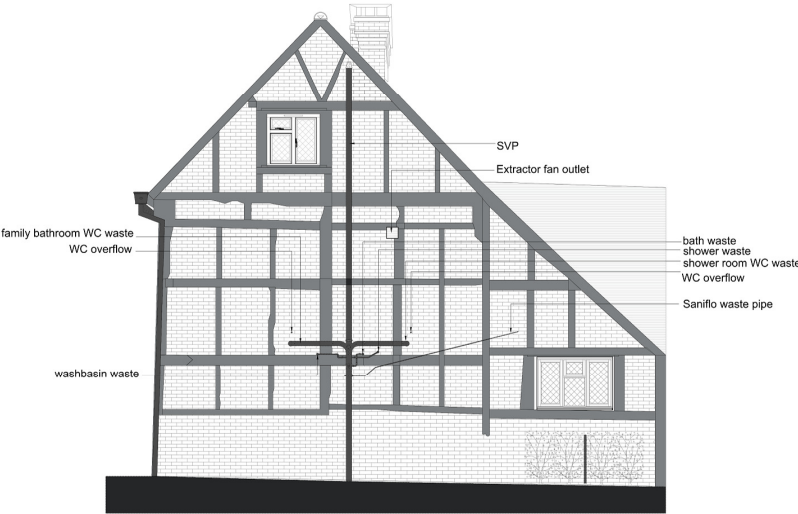
NORTH ELEVATION AS EXISTING 1:50 scale
