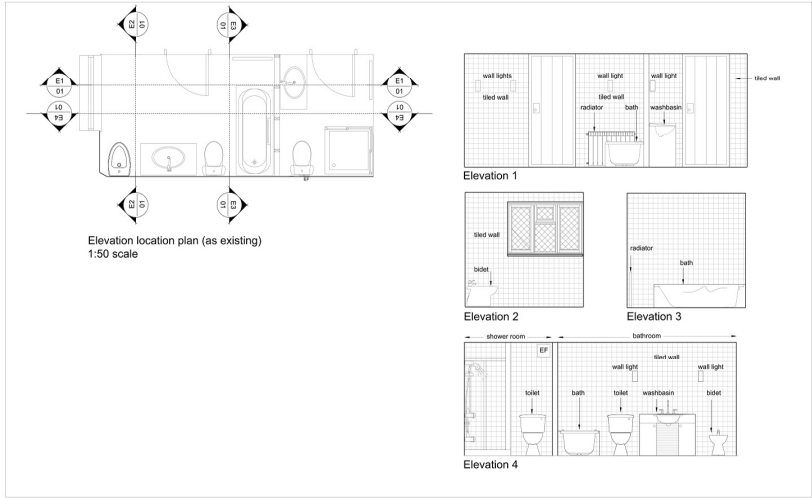
INTERNAL ELEVATIONS (FIRST FLOOR BATHROOM) AS EXISTING 1:50 scale
