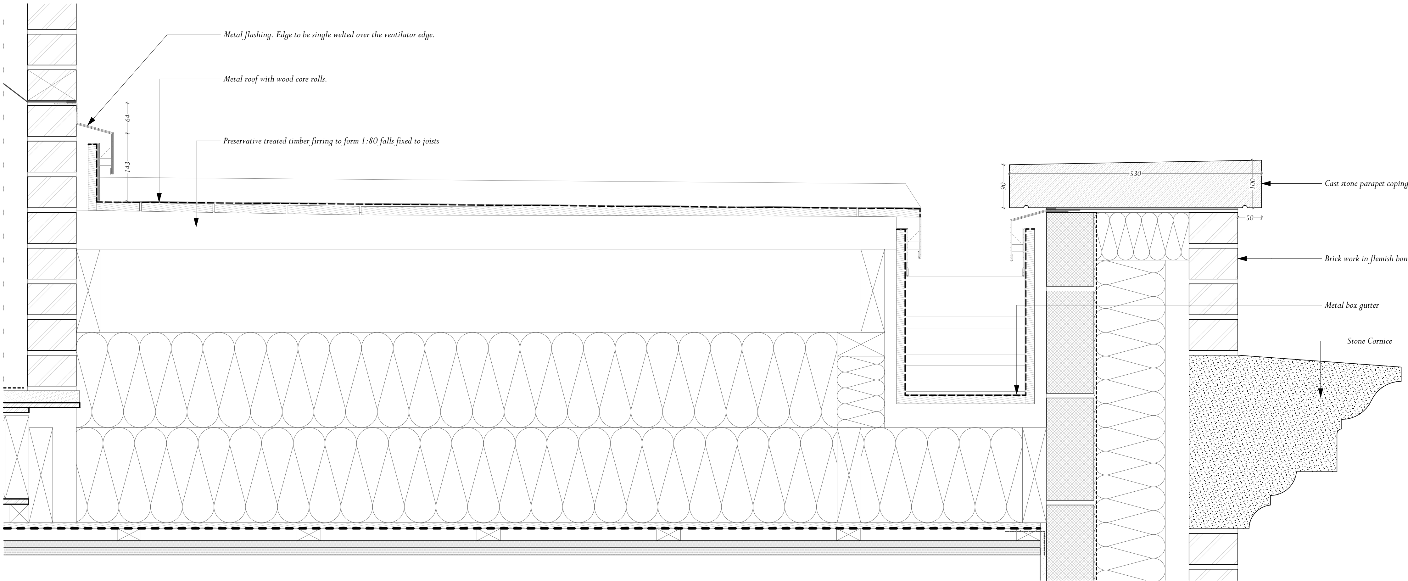
Main House Bay Window Parapet Detail (1:5)
