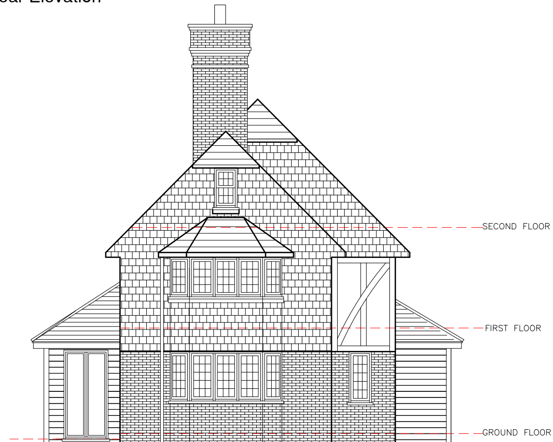
C) Existing Rear Elevation
