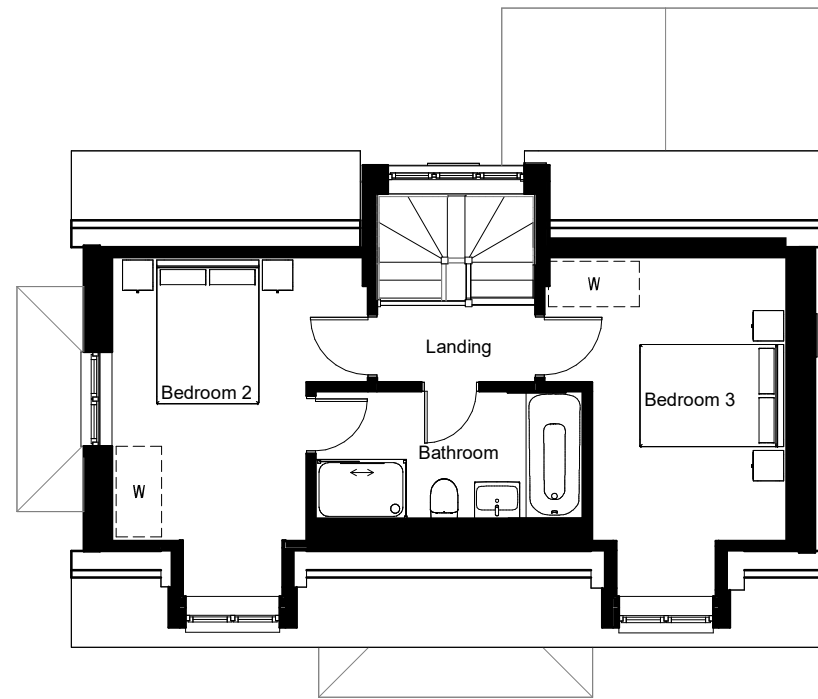
Second Floor
