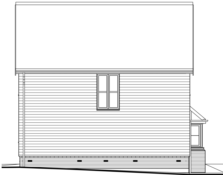
Left Elevation
