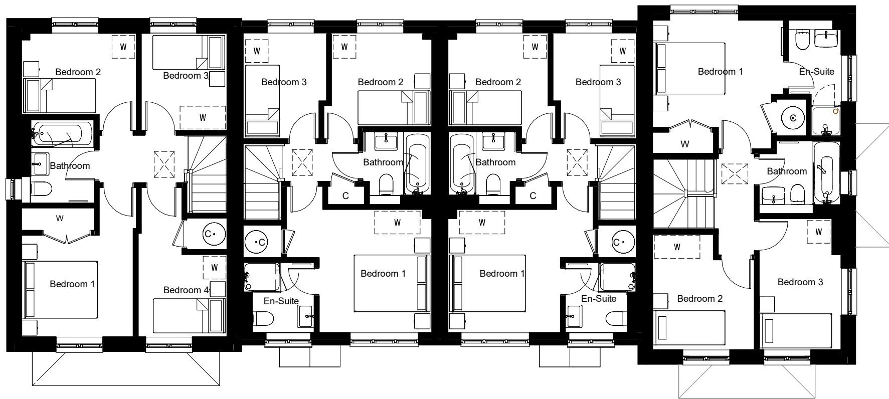
First Floor
