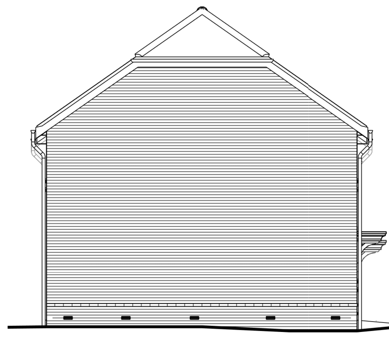
Left Elevation
