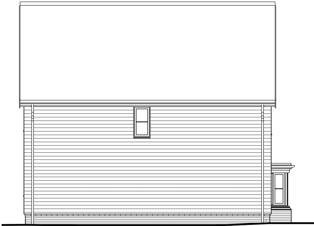
Left Elevation
