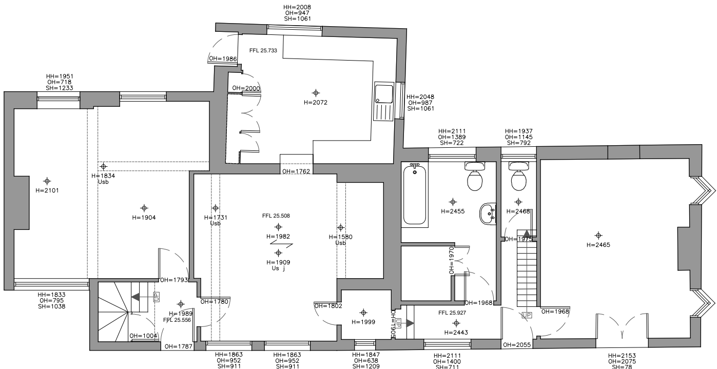
Ground Floor
