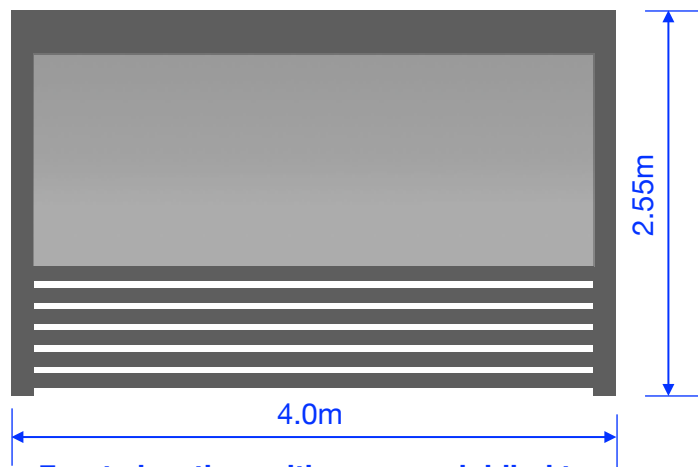
Front elevation, with grey mesh blind to front and anthracite louvres to the rear (Shown with blind partially pulled down)
