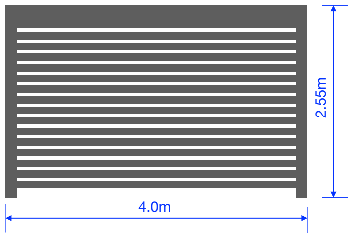
Rear elevation, with anthracite louvres
