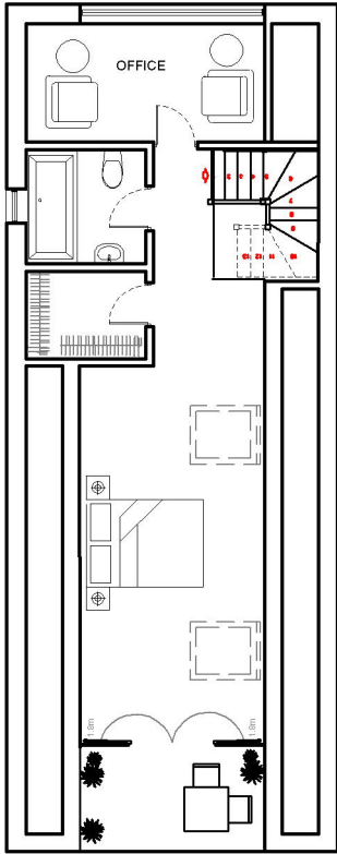
FIRST FLOOR PLAN 1:100 @A3
