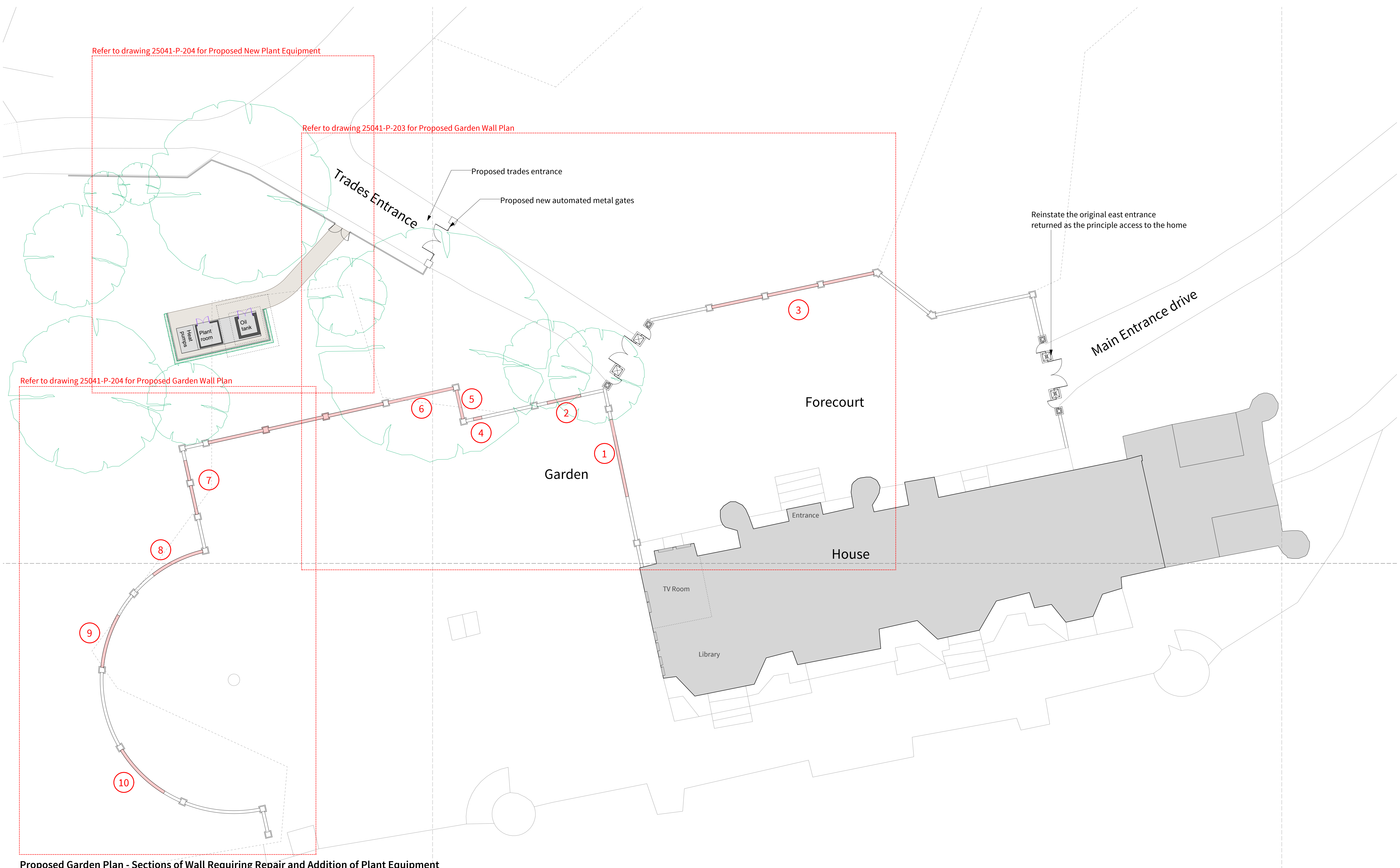
Proposed Garden Plan - Sections of Wall Requiring Repair and Addition of Plant Equipment 1:200 @A1
