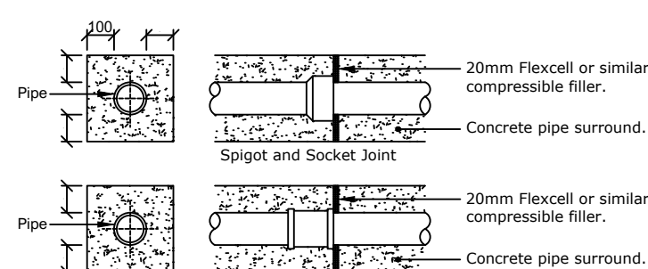
Joints For Concrete Encased Pipes (1:25)
