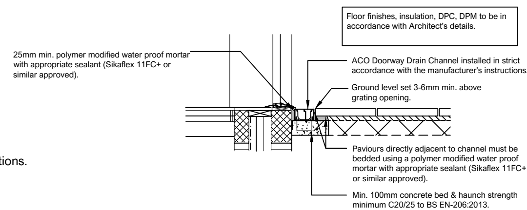
Typical Threshold Drain Detail (1:25) Patio door drain channel similar detail.
