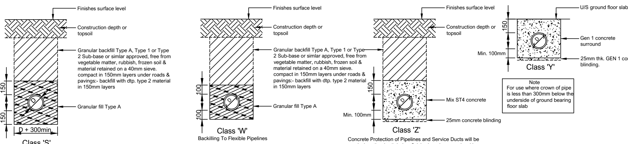
Typical Pipe Bedding Details (1:25)
