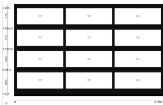
Manufacturer's proposed glazing layout (4 horizontal sections x 3 glazed panels)
