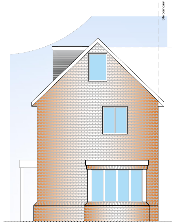
02 Rear Elevation - As Proposed 3001 1:100 (at A3)
