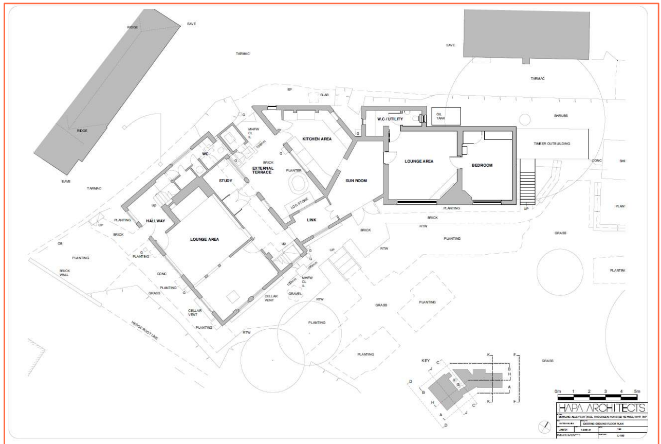
Figure 3: Existing ground floor plan (Source: HAPA Architects)
