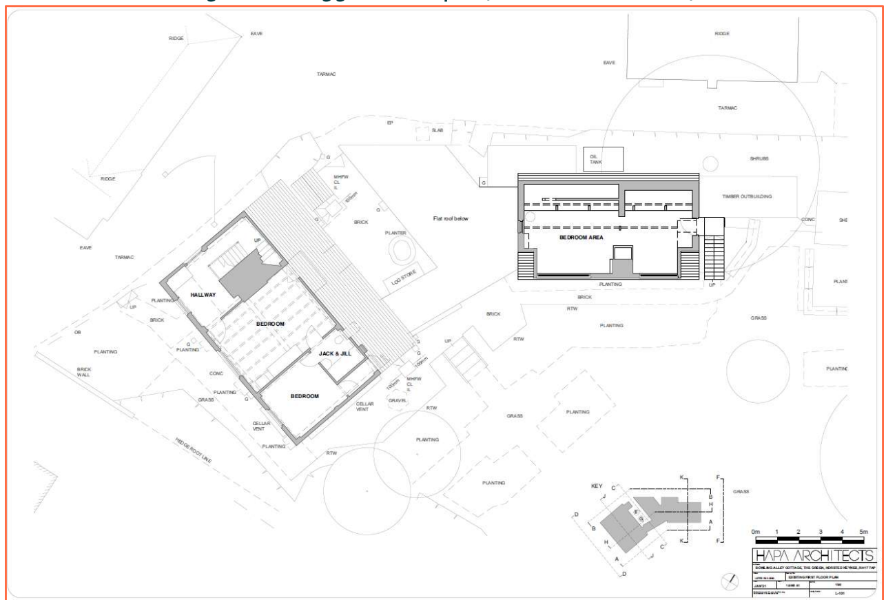
Figure 4: Existing first floor plan (Source: HAPA Architects)
