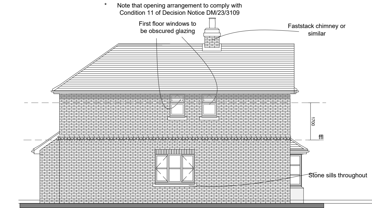
EAST ELEVATION
