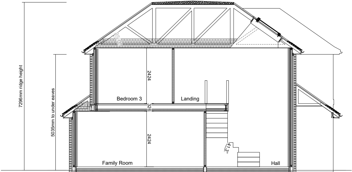
Basic section A-A
