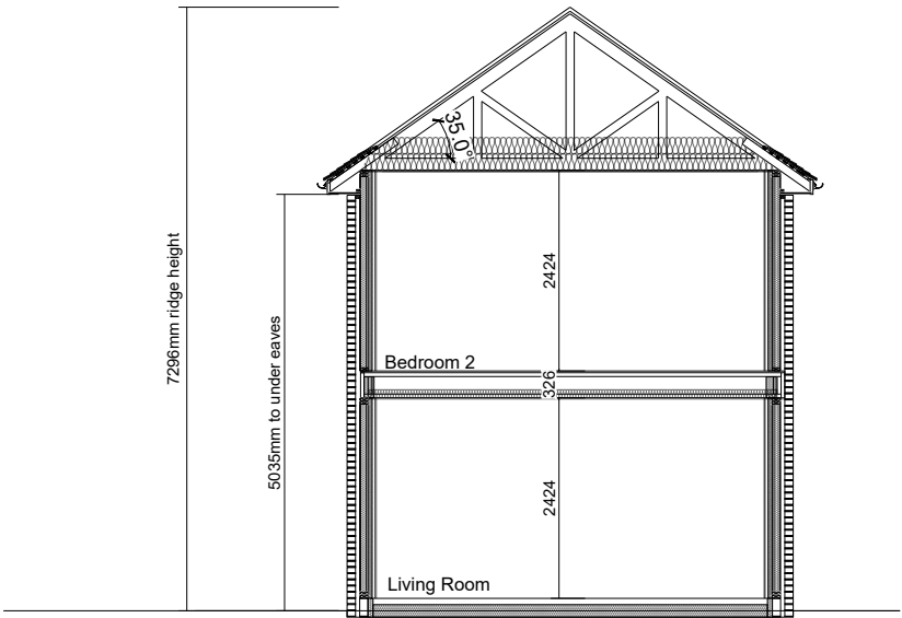
Basic section B-B
