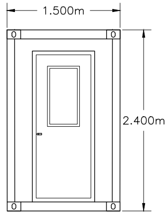
FRONT ELEVATION
