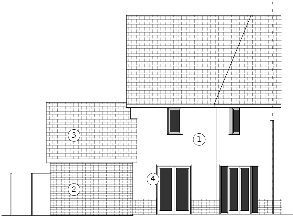
3 Rear (east facing) elevation Scale: 1:100
