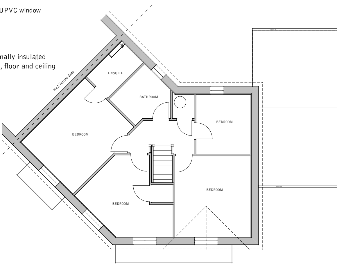
2 1F Plan Scale: 1:100 (no change)
