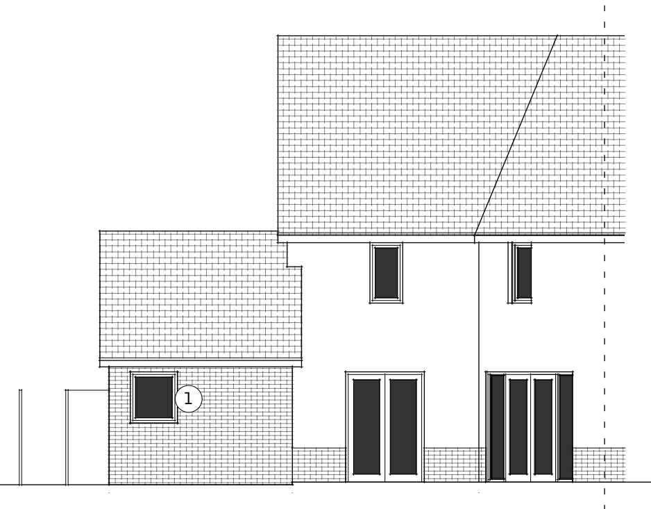
3 Rear (east facing) elevation Scale: 1:100 0 1 2 3 4 5 m
