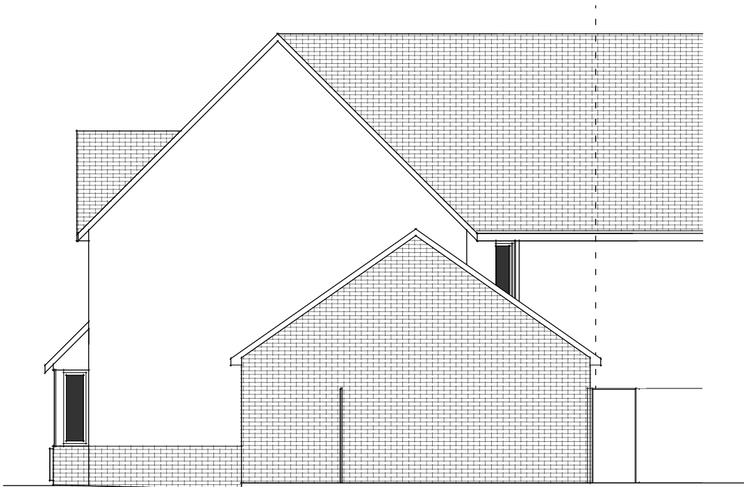
2 Side (south facing) elevation Scale: 1:100 (no change)
