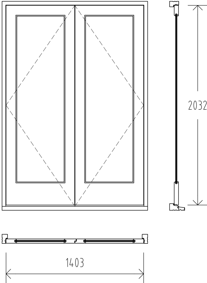
French Doors doors 1403 (w) x 2032 (h)
