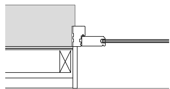
French Doors - Jamb Detail
