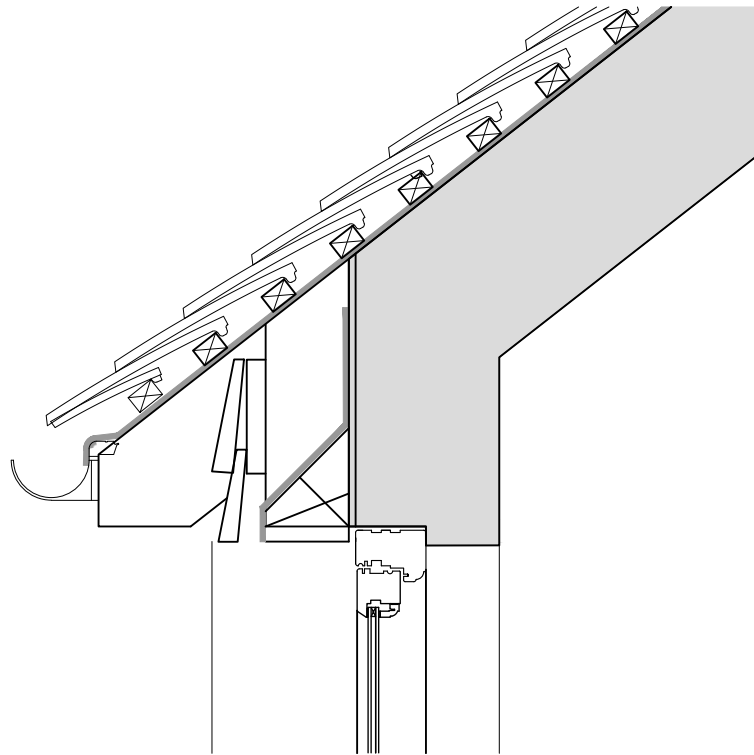
Window - Head Detail
