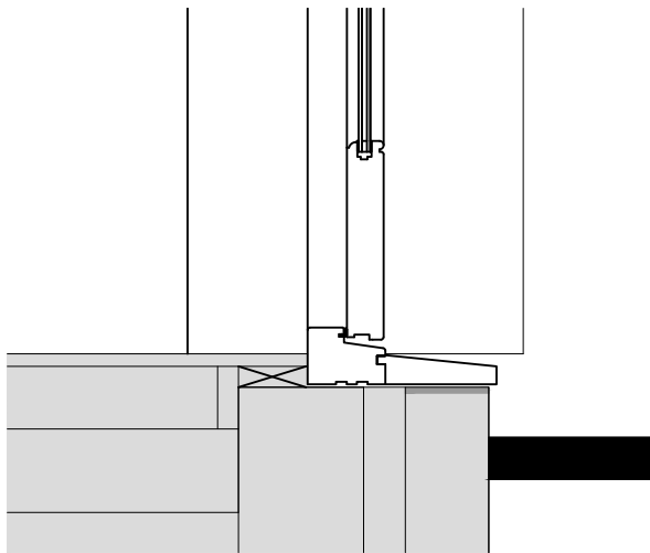
French Doors - Cill Detail
