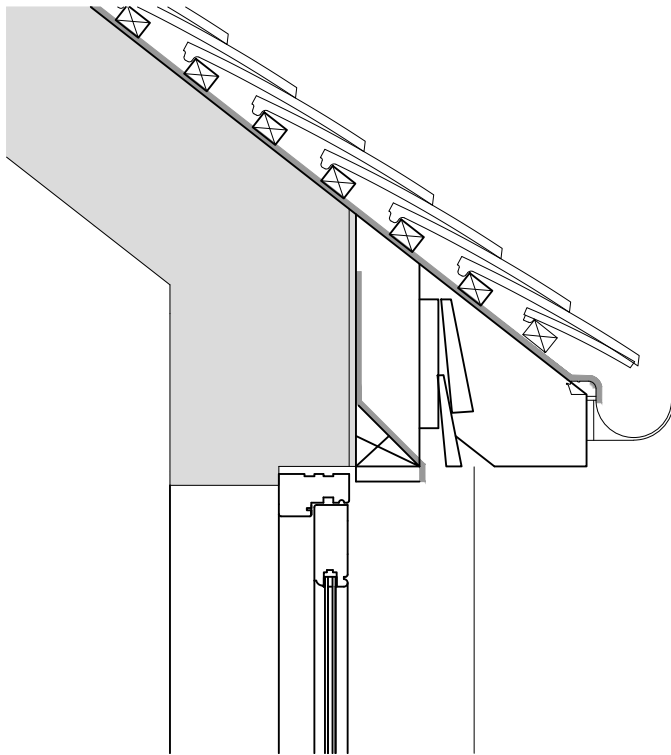
French Doors - Head Detail
