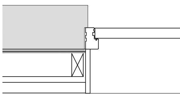
Side Entrance Door - Jamb Detail
