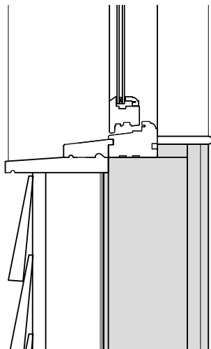
Window - Cill Detail
