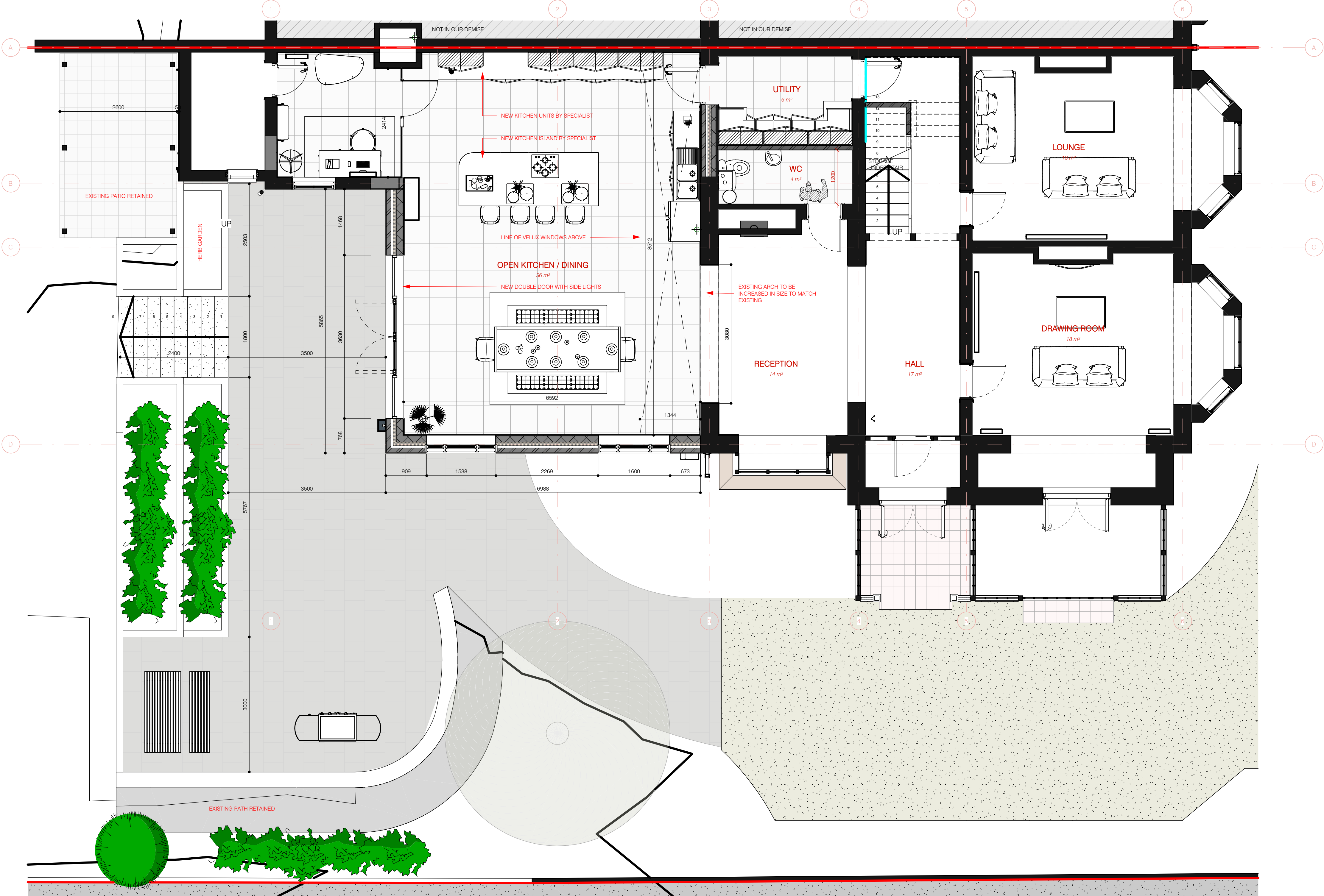
1 301005 GROUND FLOOR PLAN 1 : 50
