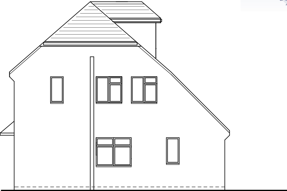
right side (northeast) elevation
