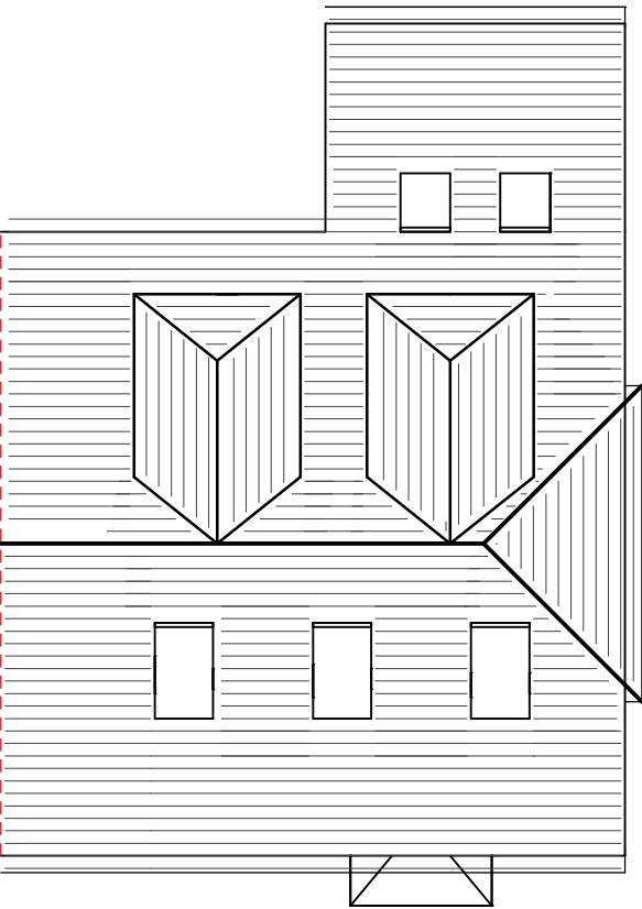
ROOF PLAN
