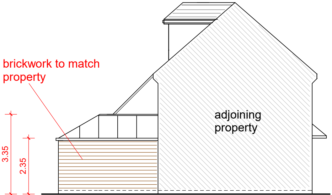
left side (southwest) elevation
