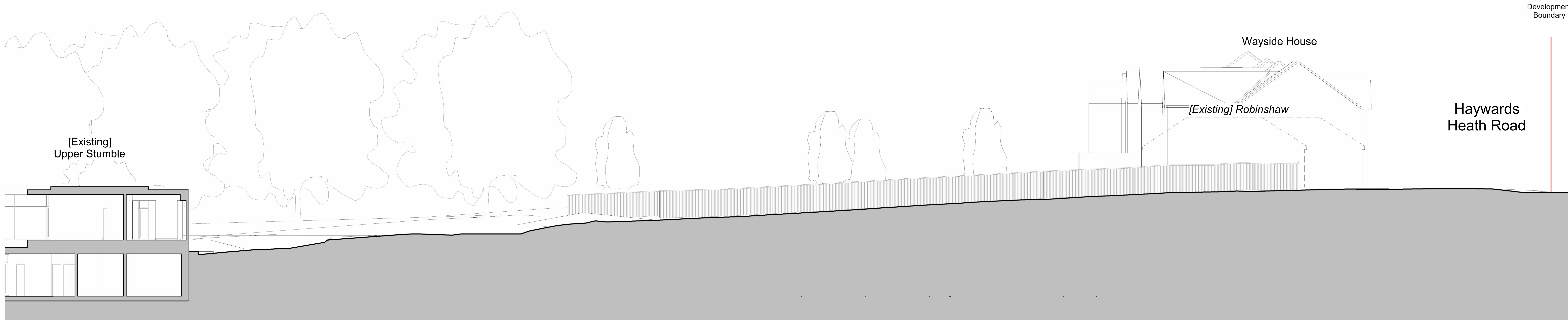
East-West Site Section B-B [Entrance Roadway] 1 : 100
