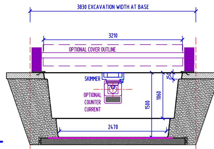
Section B - B Scale 1-50
