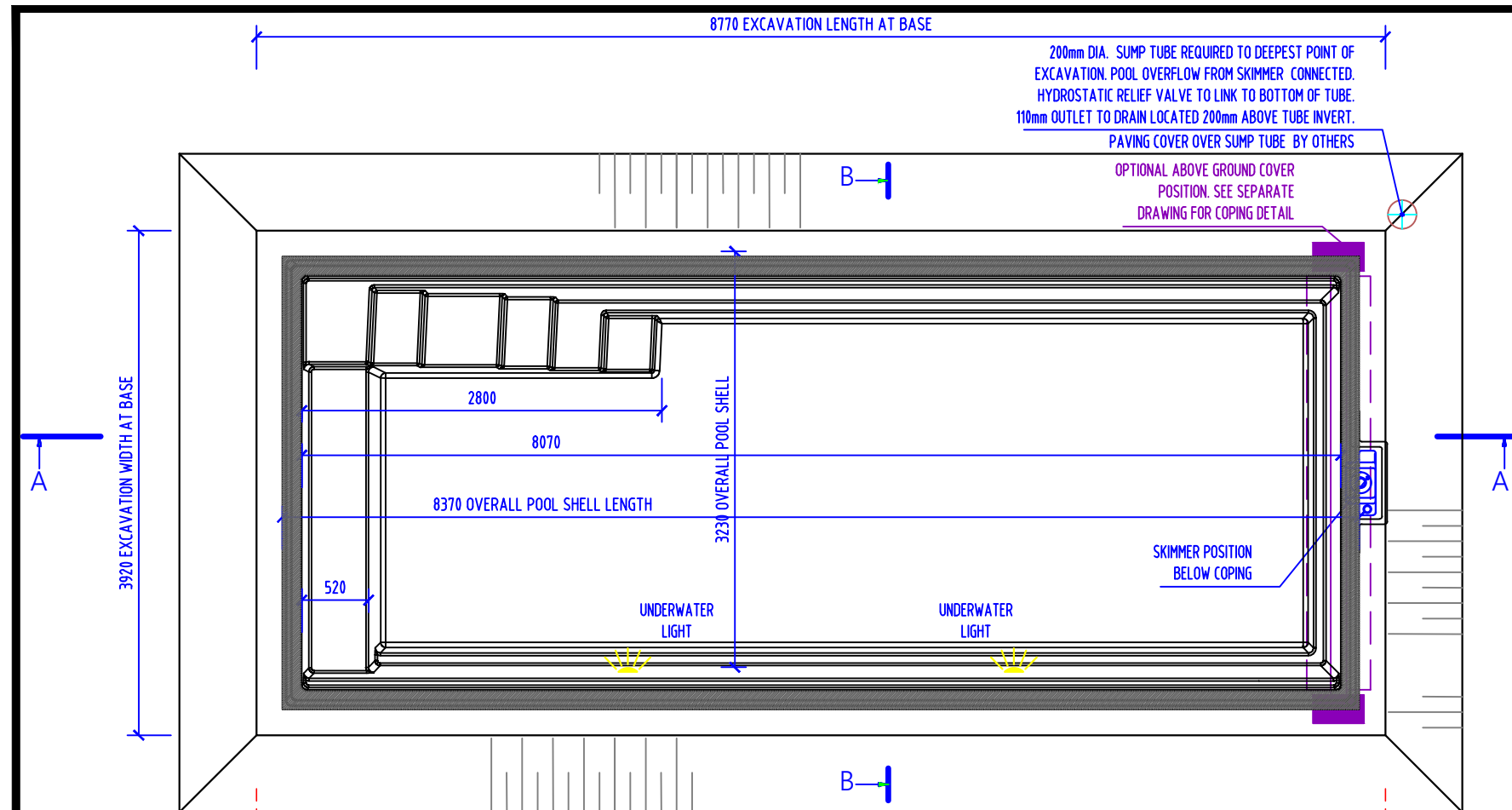
Pool Excavation Plan Scale 1-50
