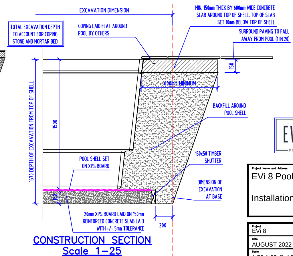
COPING SECTION Scale 1-10
