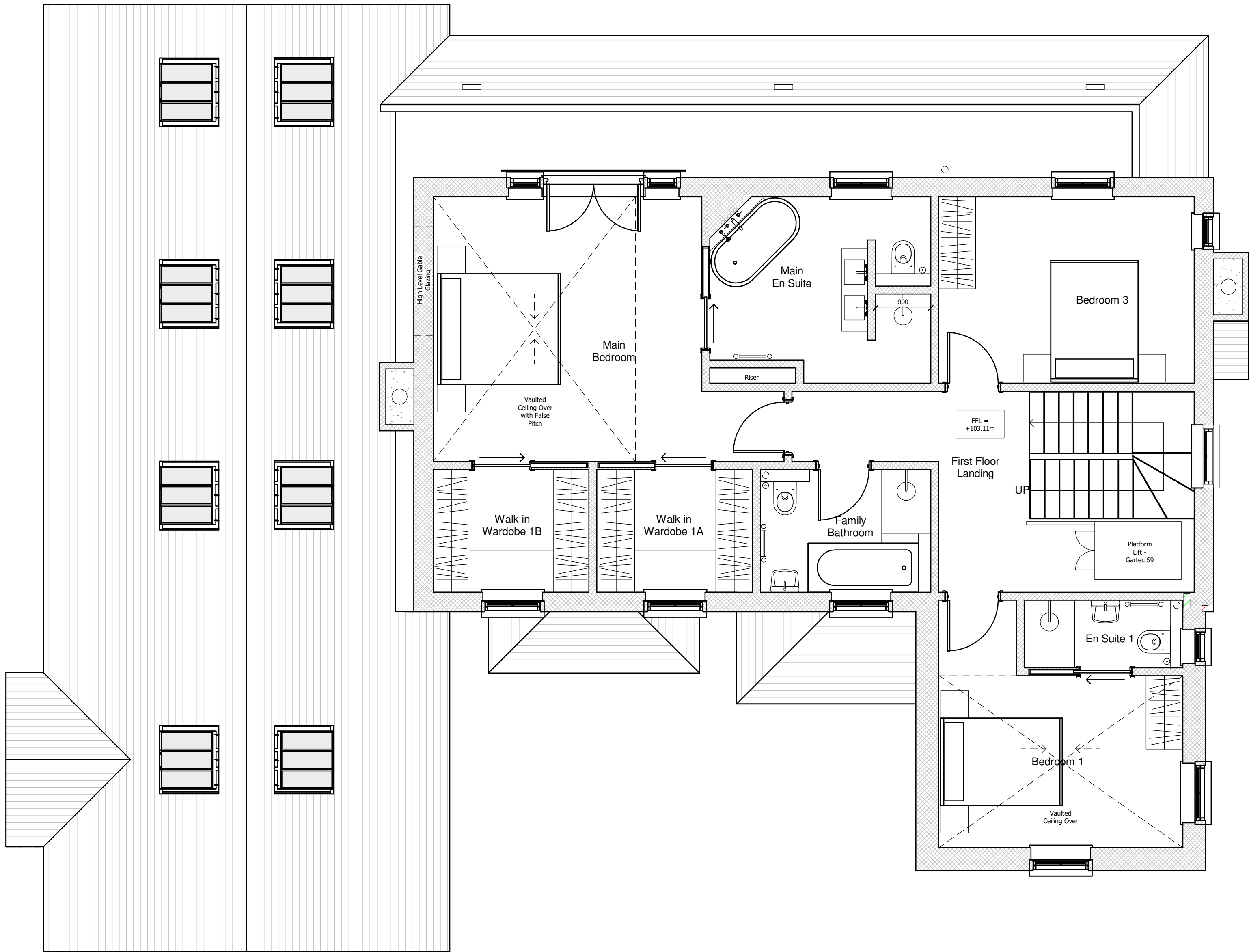
First Floor 1 : 50
