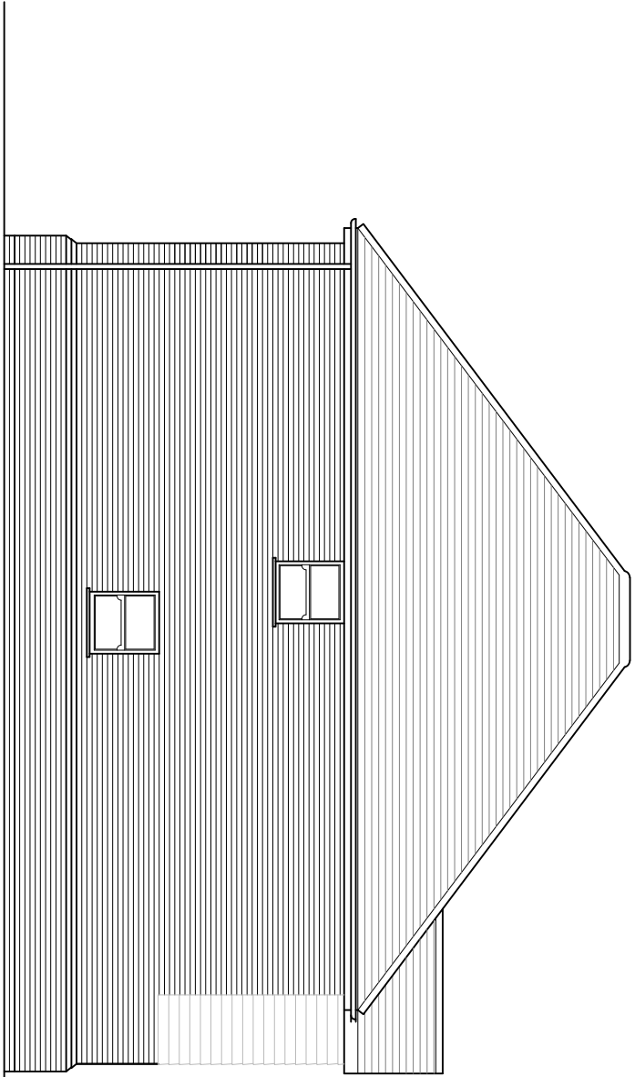
SIDE ELEVATION
