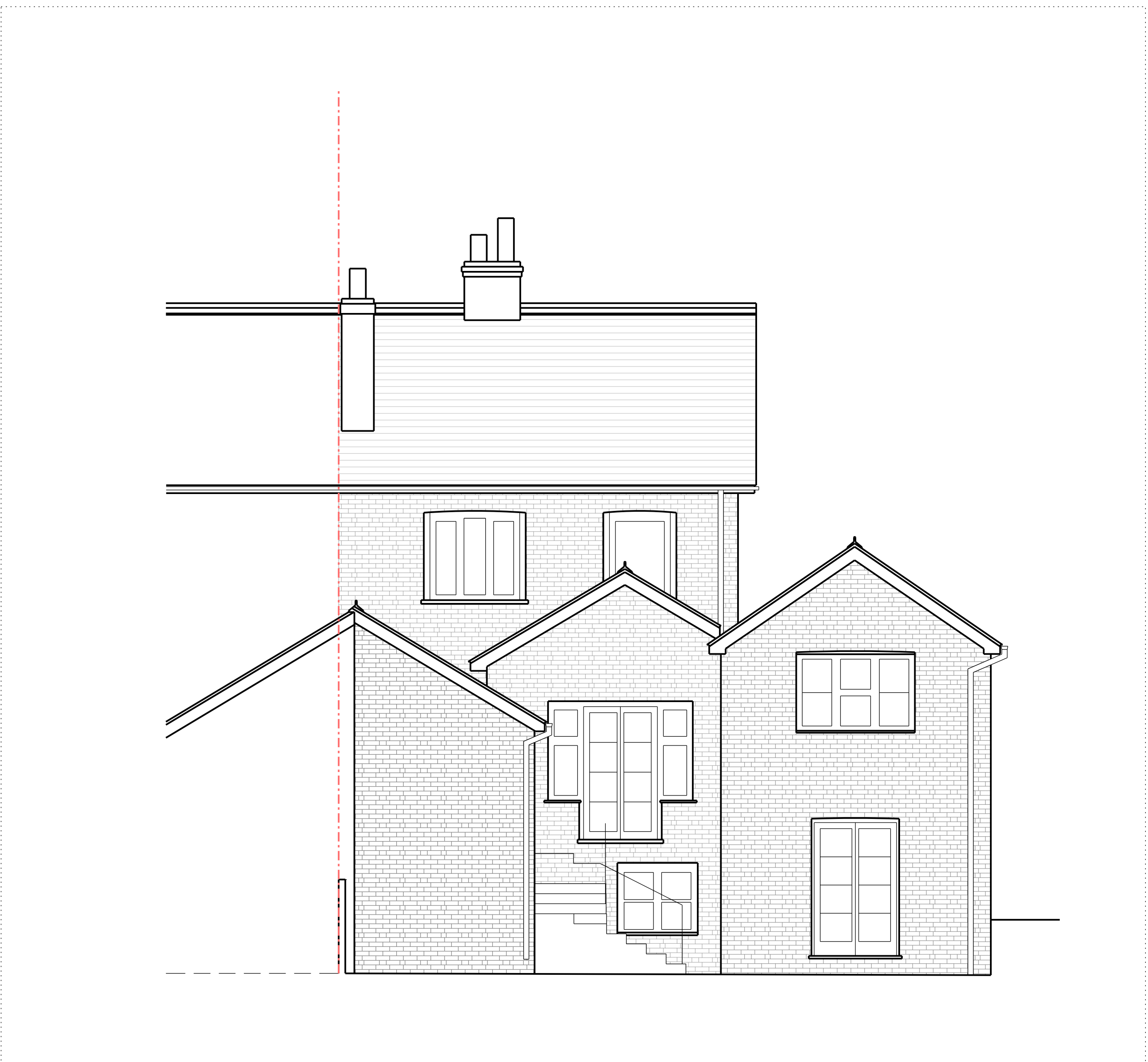
Existing Rear Elevation
