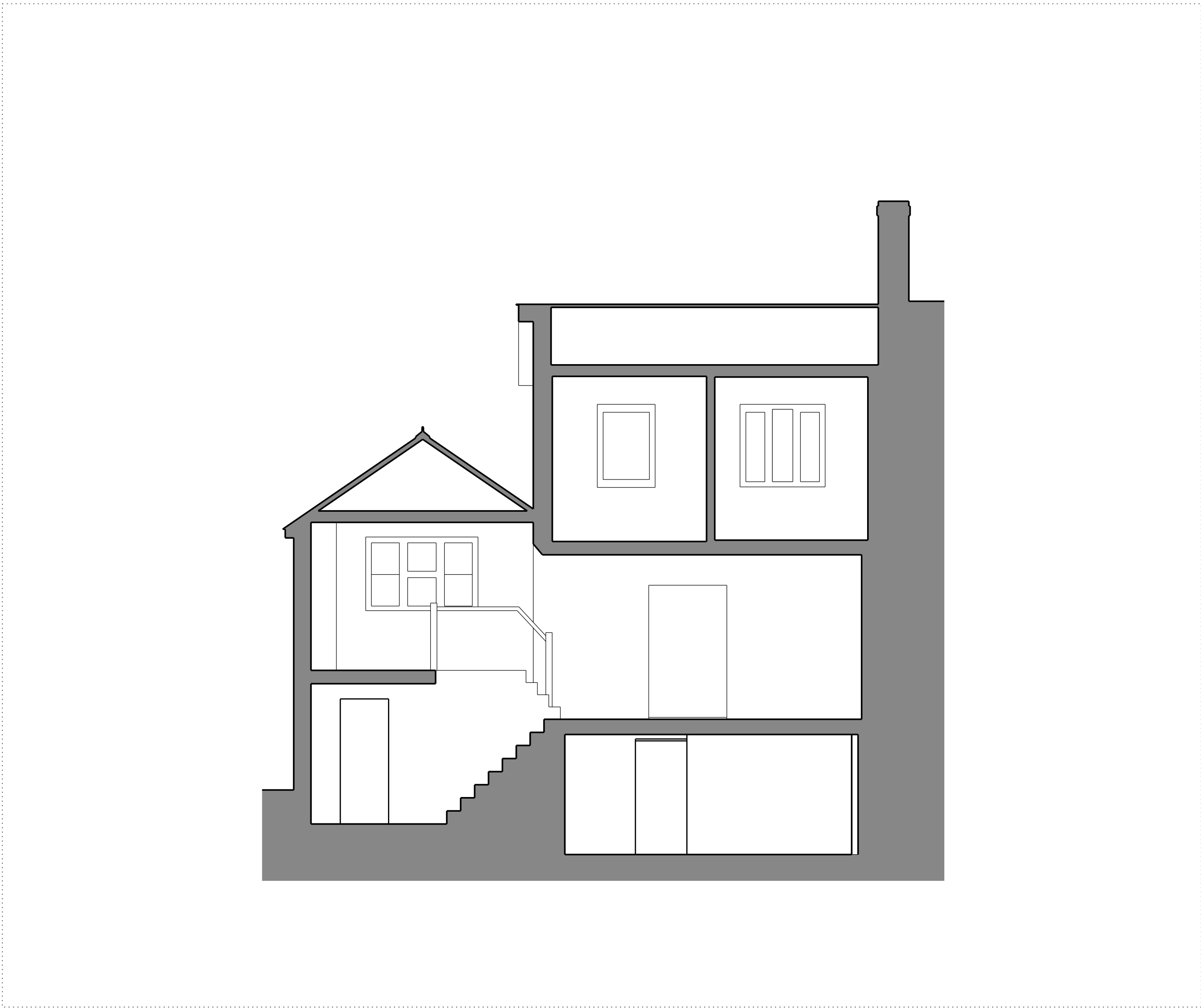
Existing Section 2
