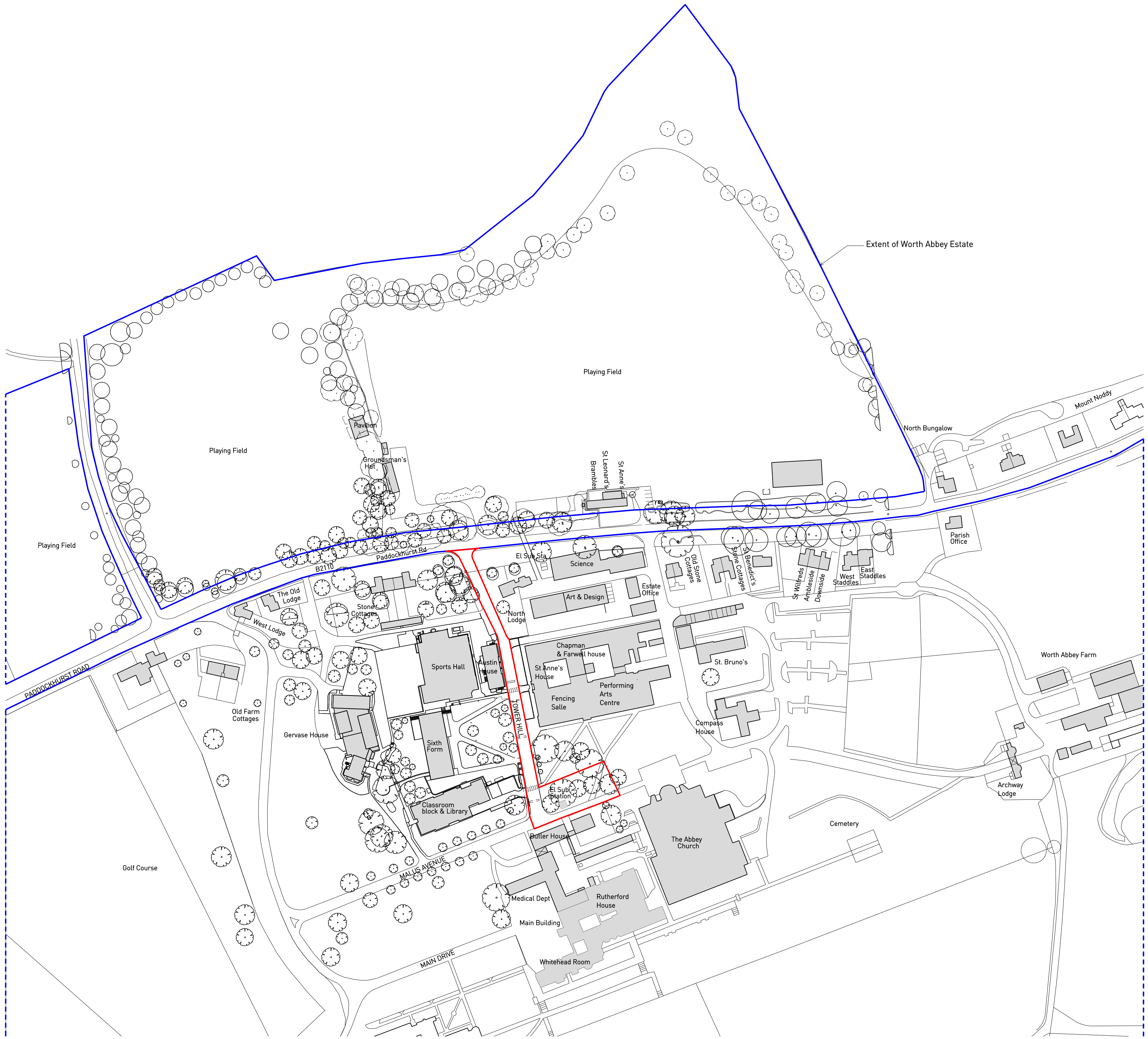
Worth School Emergency Standby Generator Base Location Plan Scale: 1:1250 at A1 /1:2500 at A3
