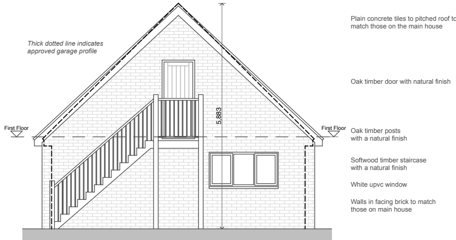
PROPOSED EAST ELEVATION 1:100
