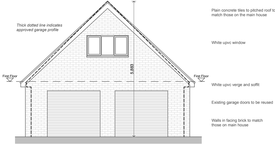
PROPOSED WEST ELEVATION 1:100
