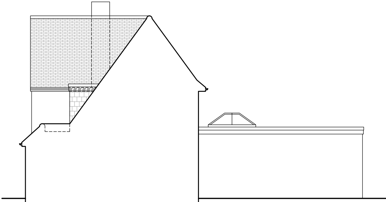
Existing RHS Elevation Scale 1/100@A3
