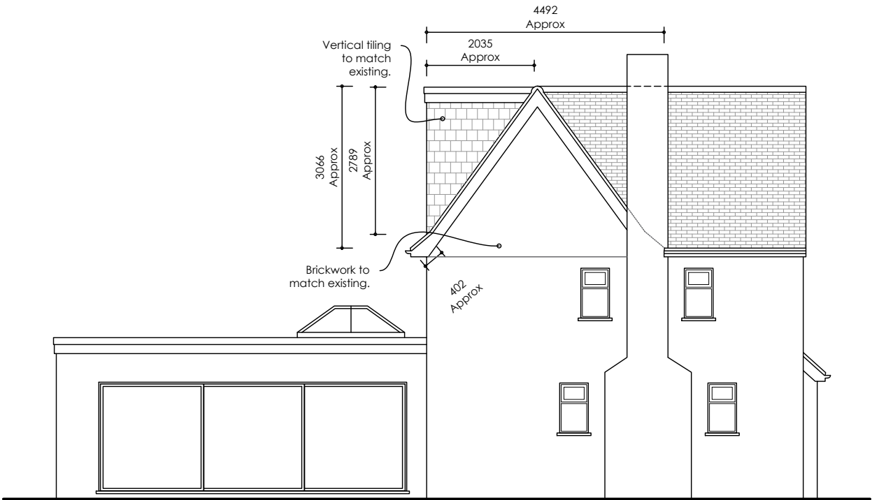
Proposed LHS Elevation Scale 1/100@A3
