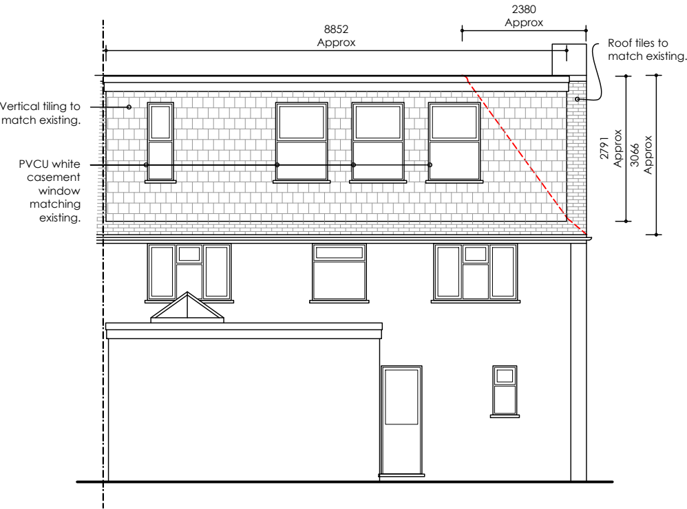
Proposed Rear Elevation Scale 1/100@A3
