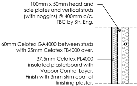
Stud Ashlar / Dwarf Wall Scale 1/20@A3
