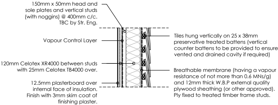
Dormer Construction Scale 1/20@A3
