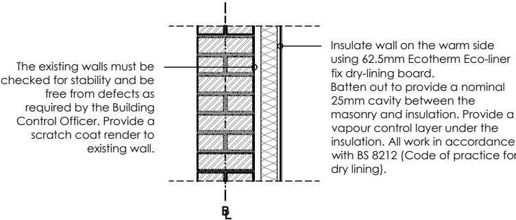
Upgrading Solid Party Wall (cold adjoining space) Scale 1/20@A3
