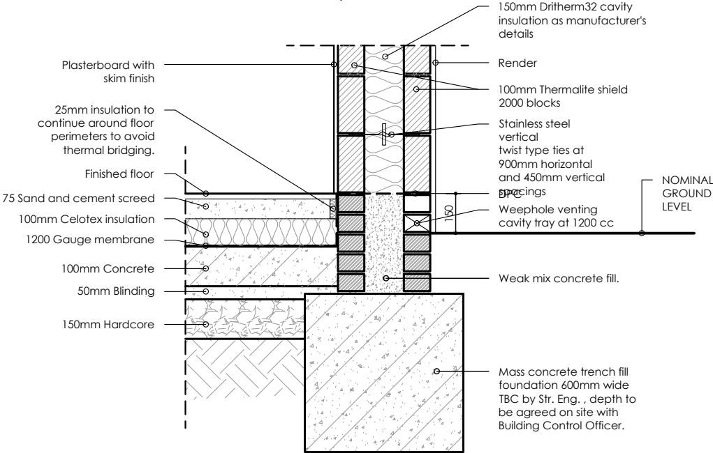
Foundation Detail for Rear Wall Scale 1/20@A3
