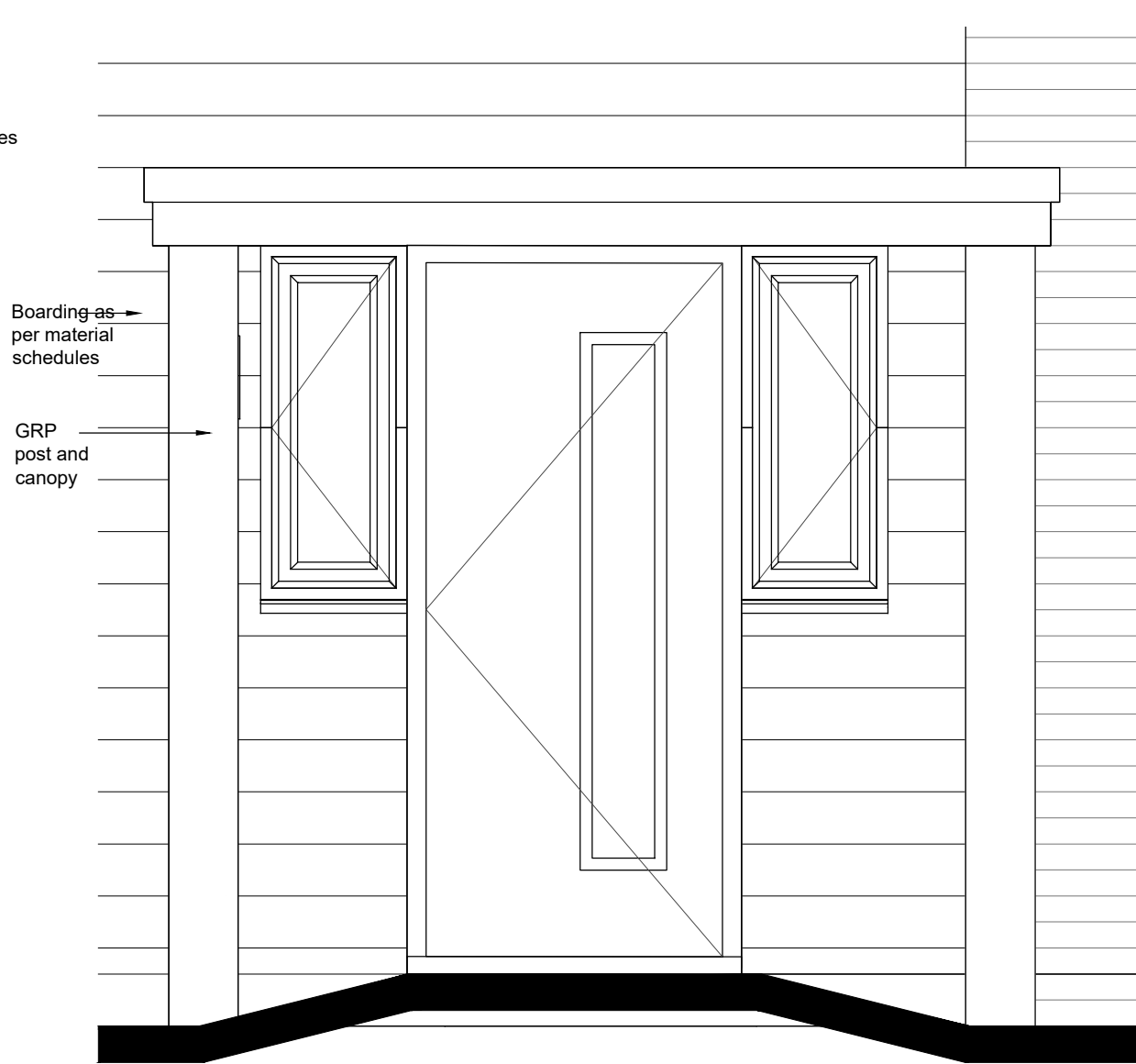
Fuller Front elevation Plots (as) 37, 82, 210, 234, 245, 247 (H) 35, 49, 73, 79, 235, 242
