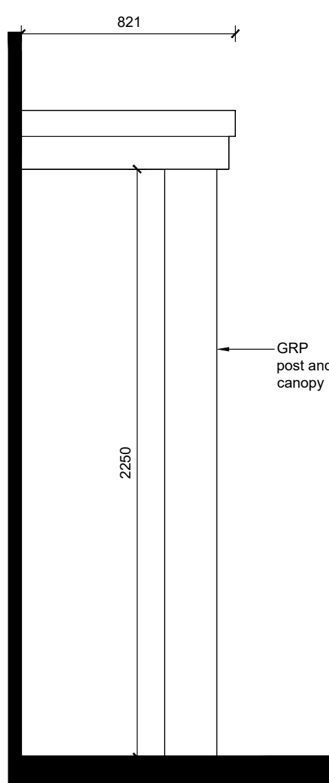
Typical canopy side elevation
