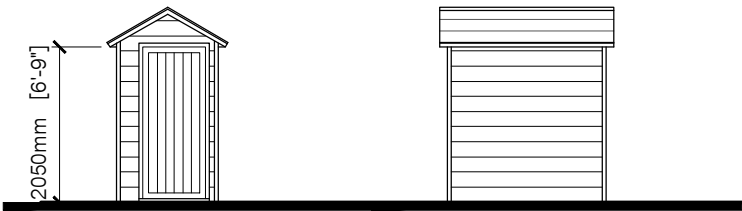
Front Elevation Side Elevations
