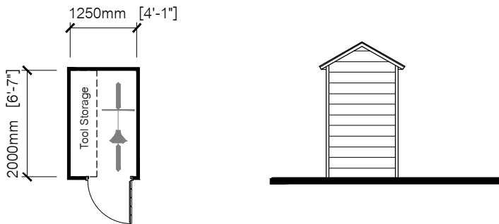
Plan Rear Elevation
