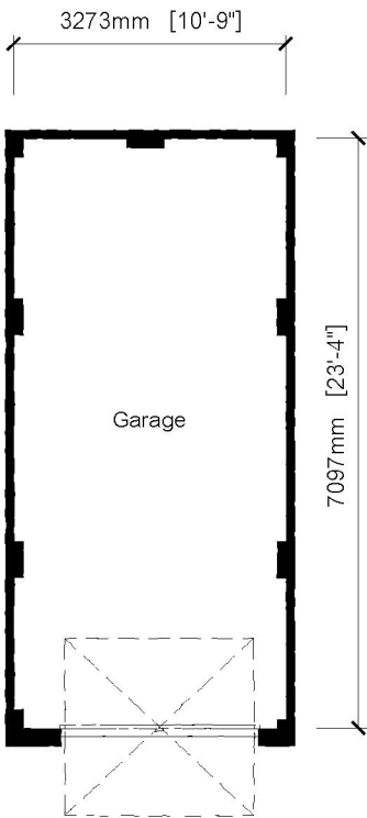
Floor Plan
