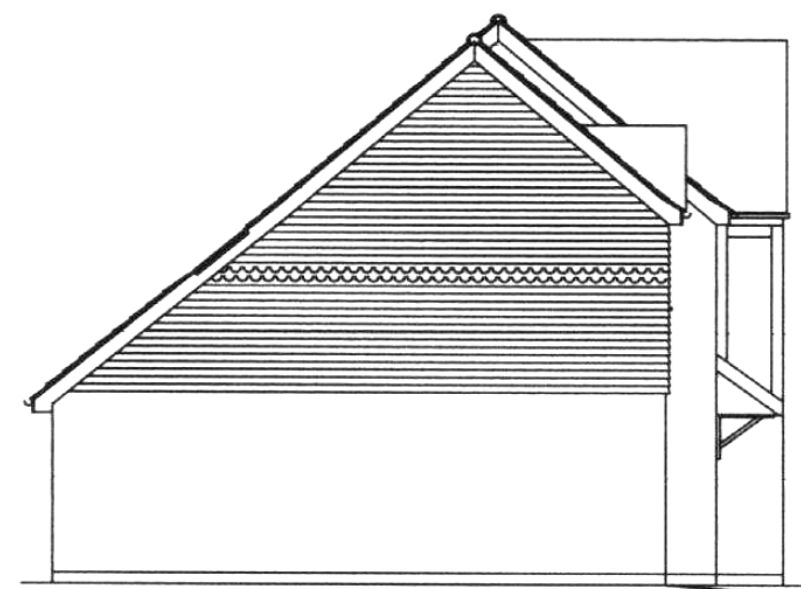
NORTH ELEVATION
