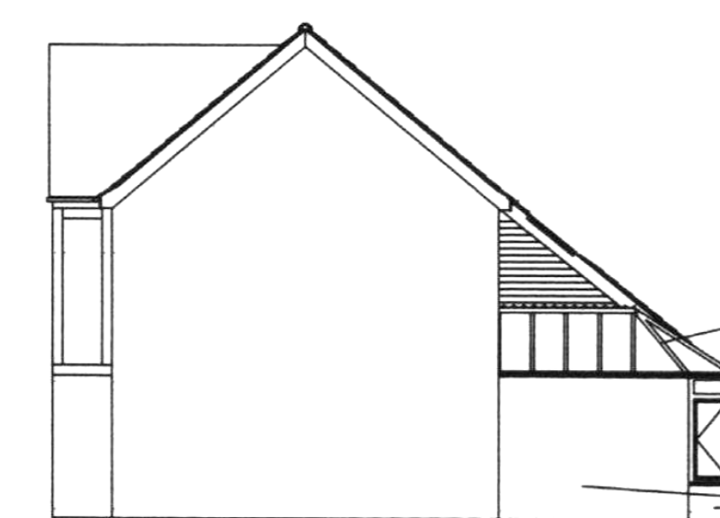
SOUTH ELEVATION
