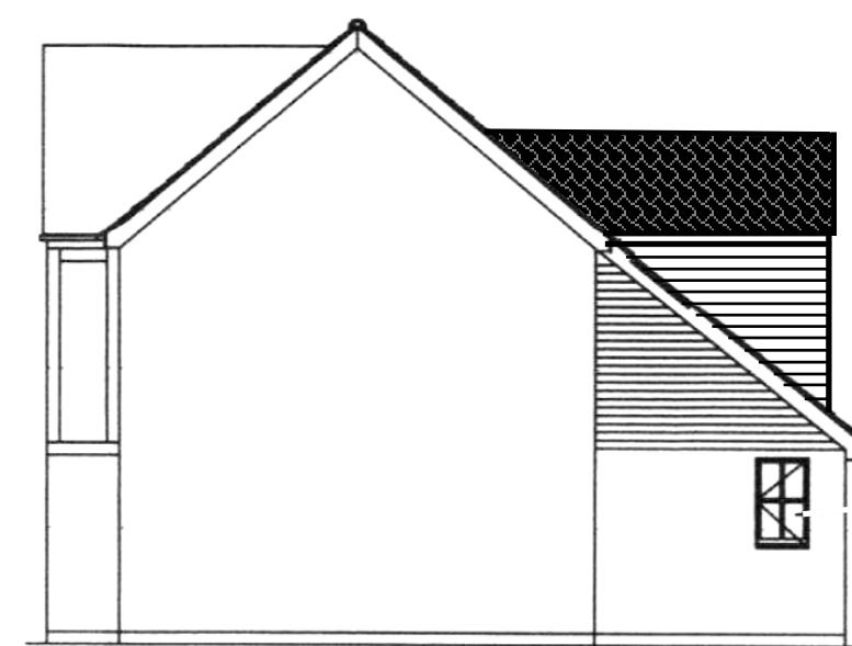
SOUTH ELEVATION
