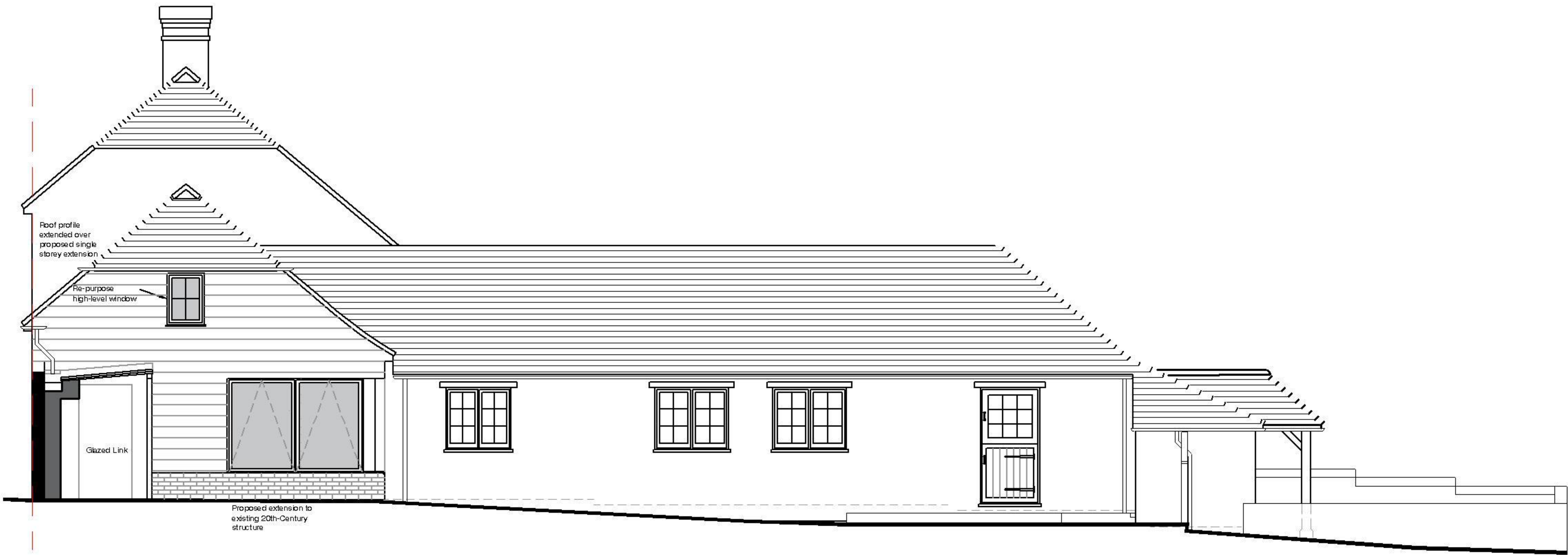
Section through Glazed Link (West View)
