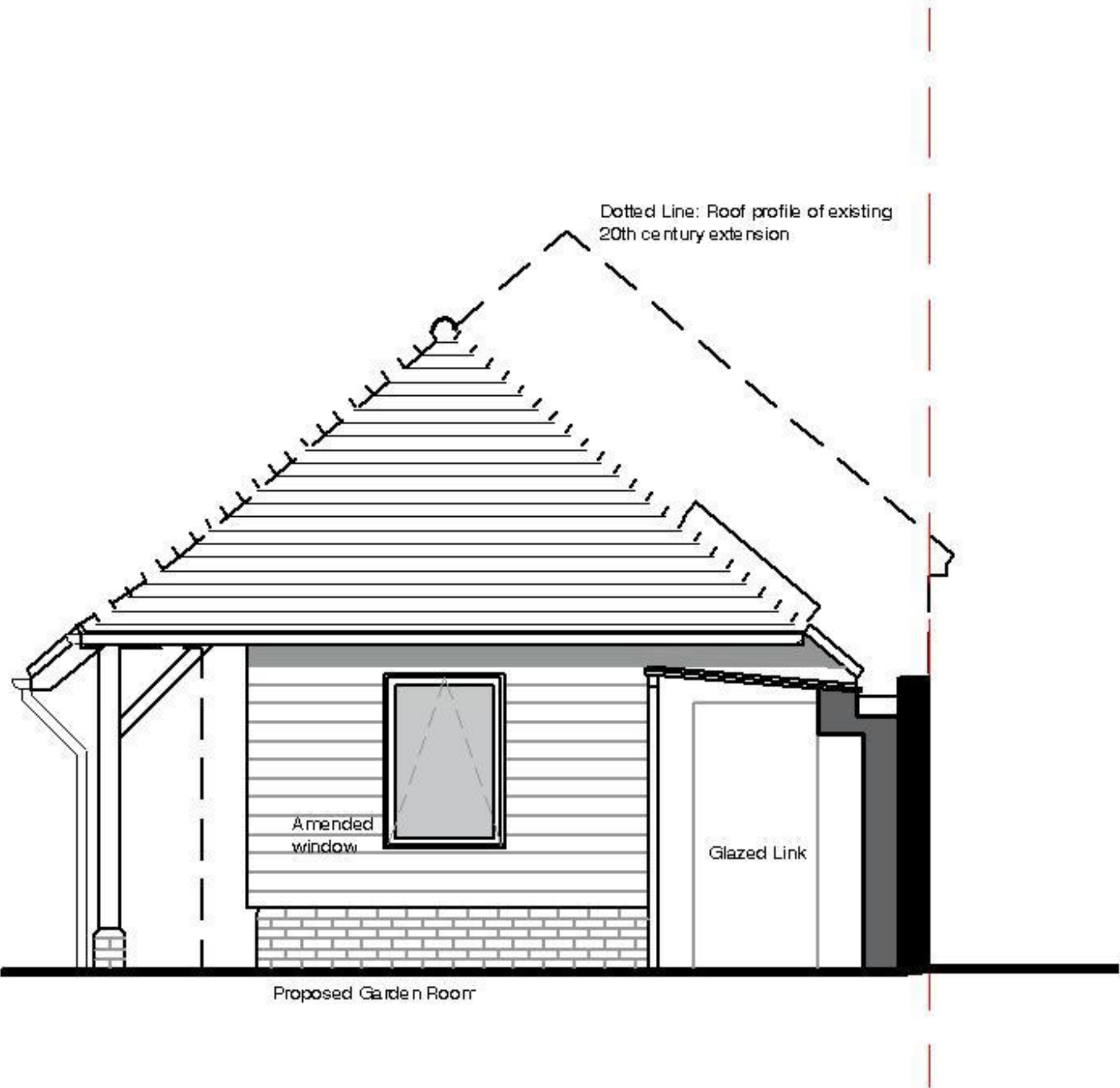
Section through Glazed Link (East View)
