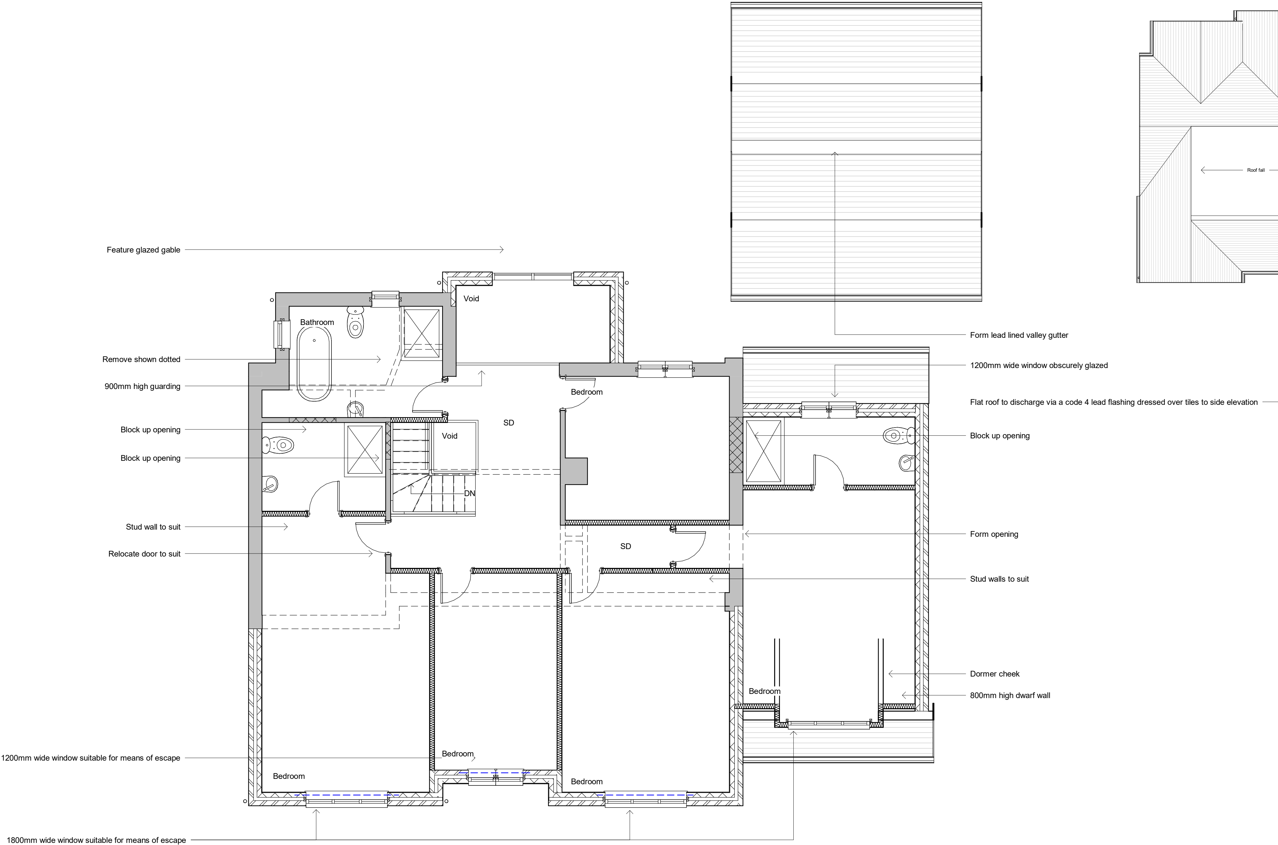
First Floor
