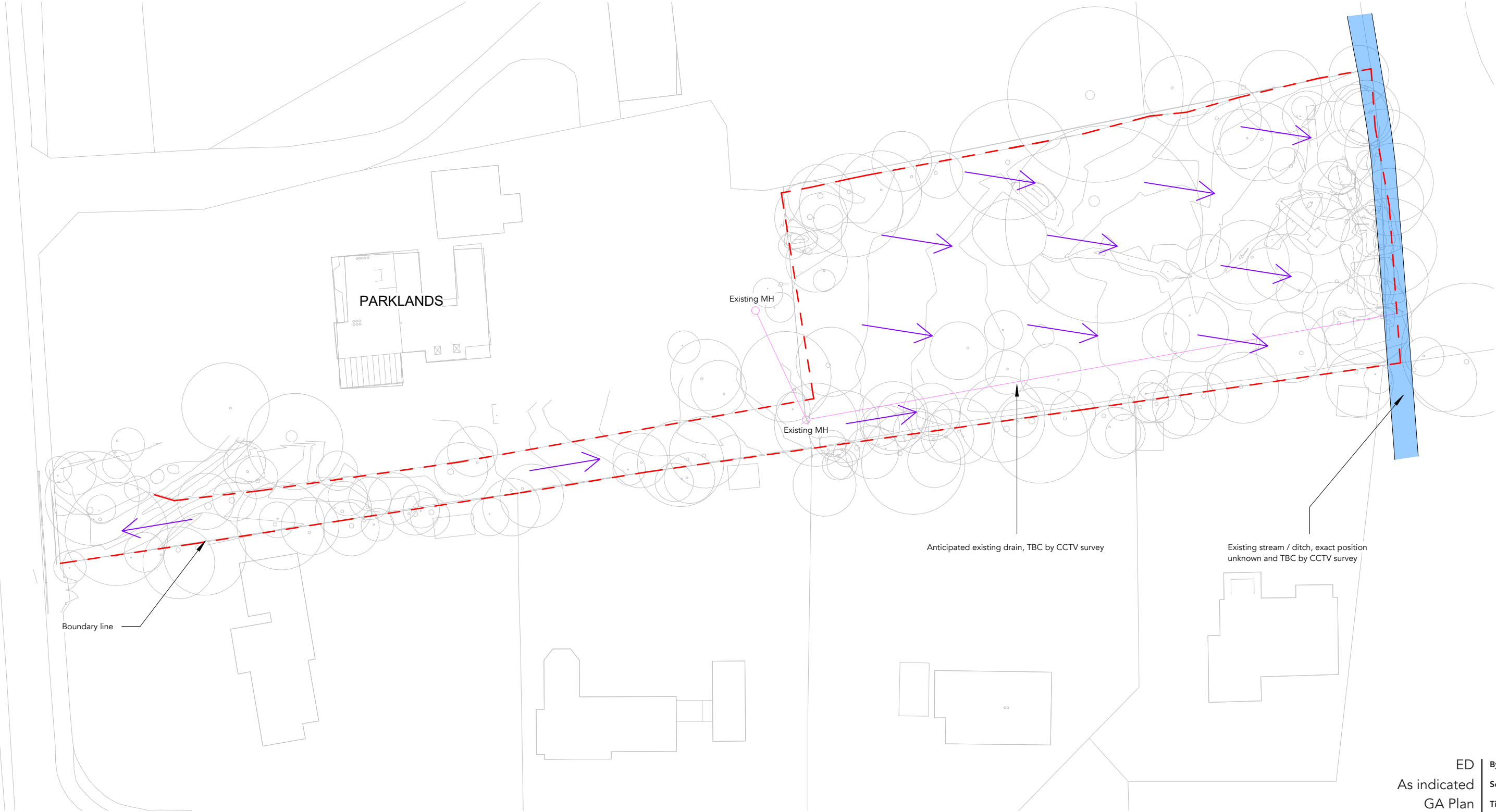
Drainage Plan - Existing
