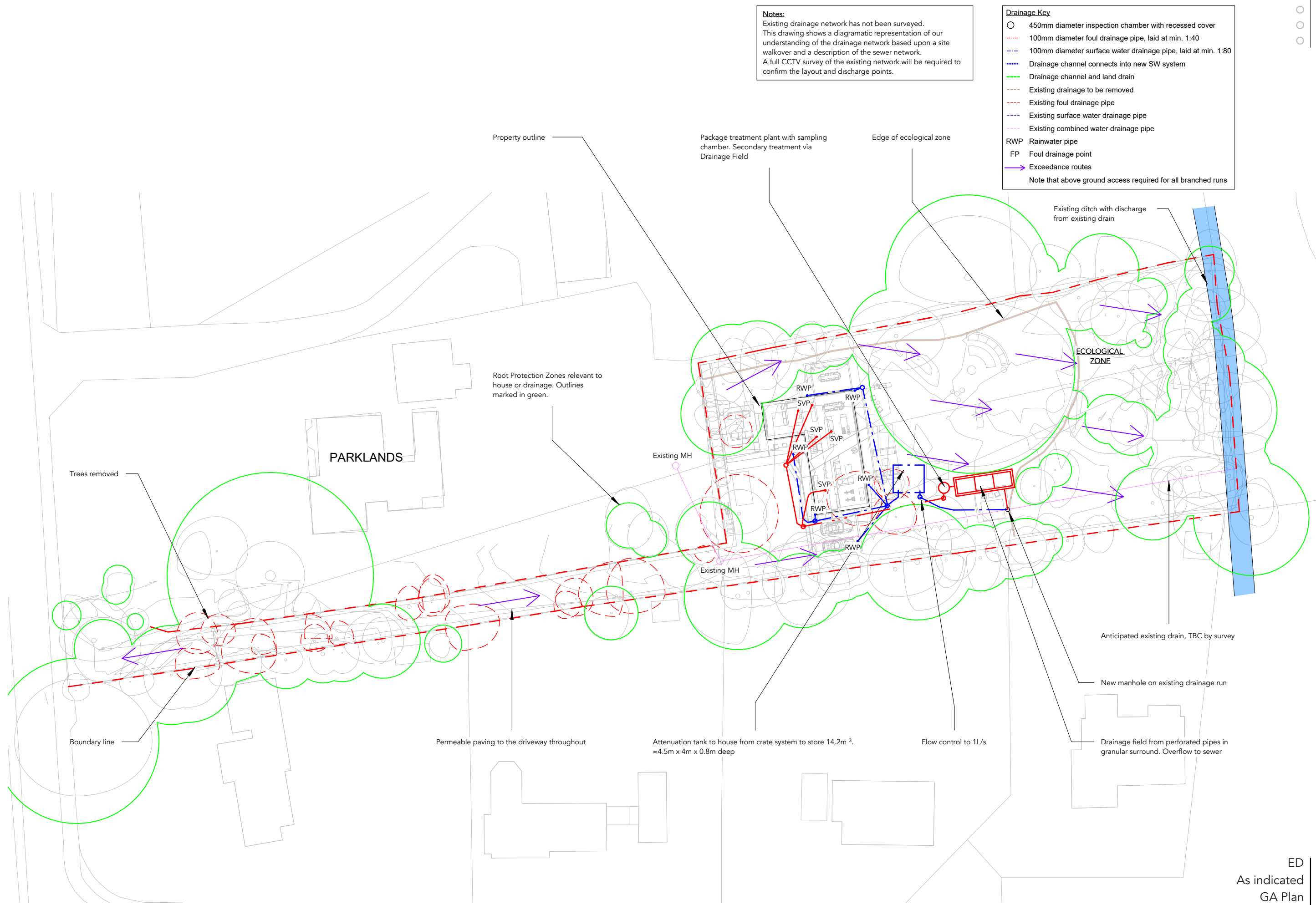
Drainage Plan - Proposed
