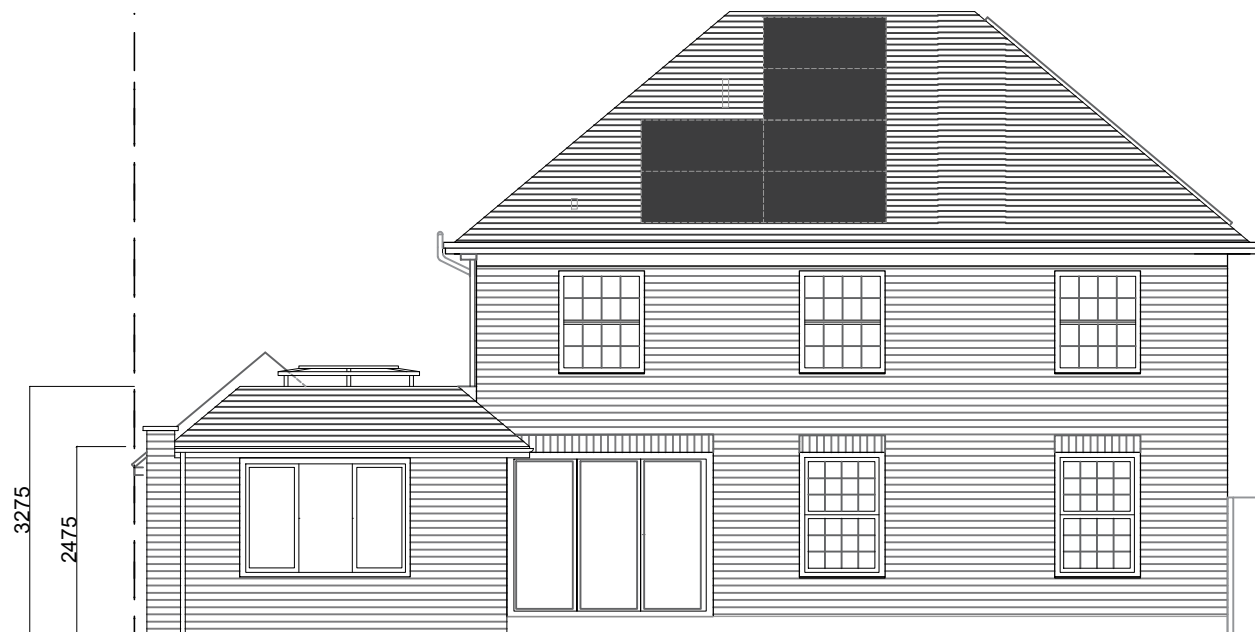
PROPOSED REAR (WEST) ELEVATION
