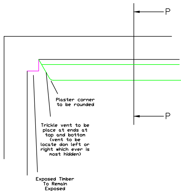
Typical Fillet 1
