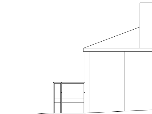
East elevation
