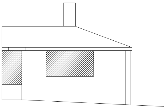
West elevation
